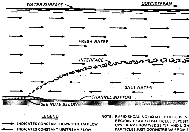
Figure 3-2. Conditions typical of highly stratified estuary
