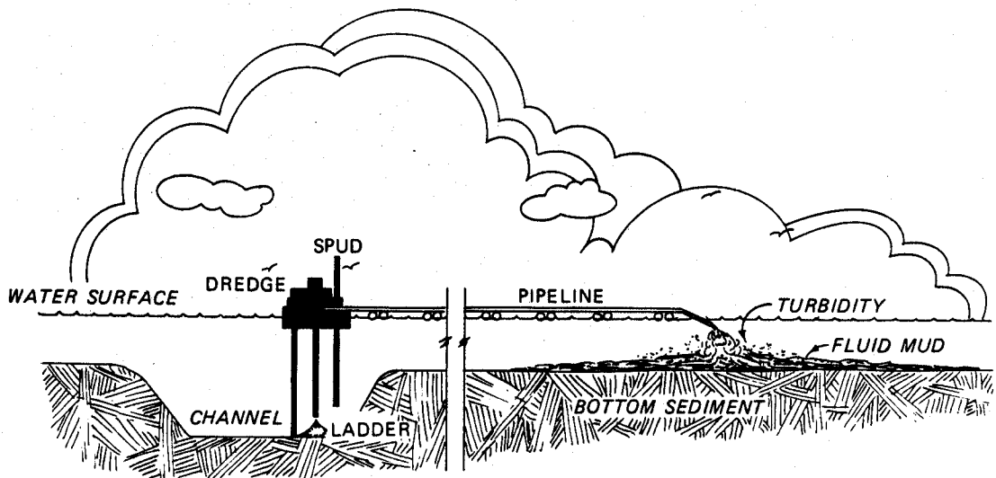
Figure 4-10. Typical channel maintenance dredging operation with open-water pipeline disposal
