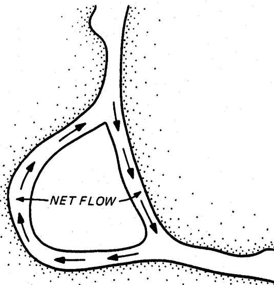
a. Residual flow pattern at an inlet
