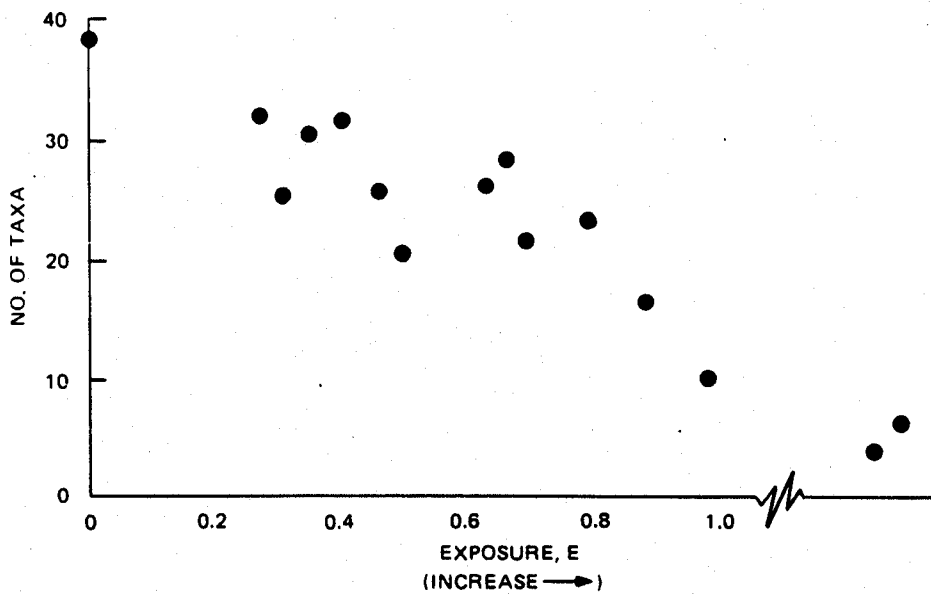
Figure 2-4. Relationship between exposure to wave action and total benthos and number of taxa, E = \log(1 + fwd^{-2}) , where f = fetch, w = fraction of time wind blew toward station, and d = depth of station
